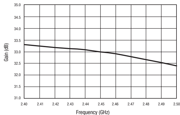
Figure 4. Typical Gain vs Frequency Response
