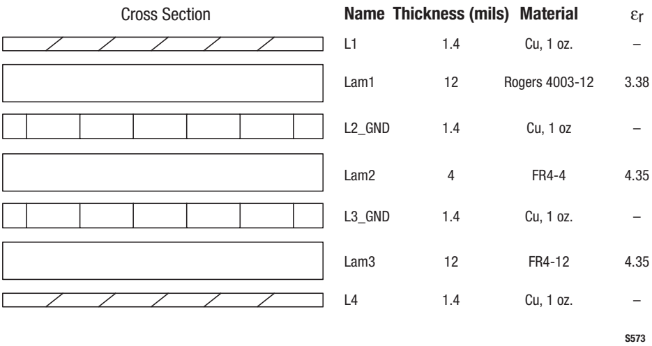
Figure 13. Layer Detail Physical Characteristics
