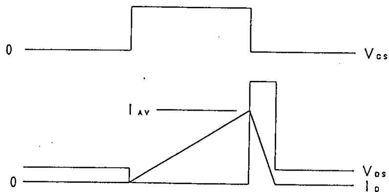
Fig.2 Operating waveforms
