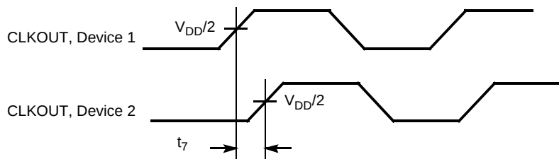
Figure 8. Device-Device Skew
