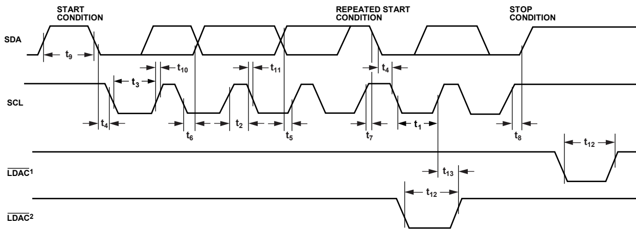
Figure 2. 2-Wire Serial Interface Timing Diagram
