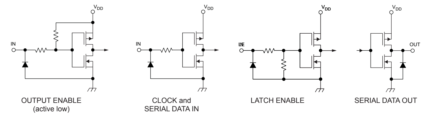
Inputs and Outputs Equivalent Circuits
