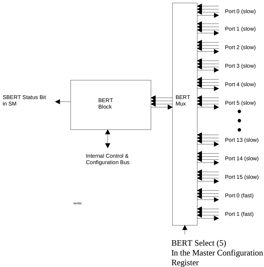
BERT Mux Diagram Figure 5.5A
