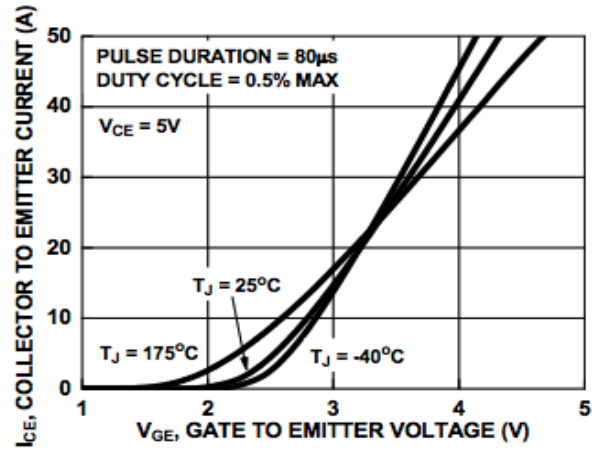
Figure 8. Transfer Characteristics
