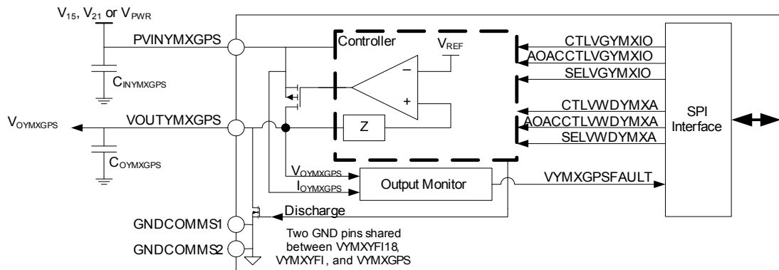
Figure 49. VYMxGPS Detailed Internal Block Diagram
