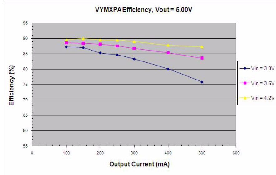
Figure 37. VYMXPAA Efficiency Curves ( V_{OYMXPAA} = 5.0\text{ V} )
