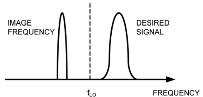
Figure 1. Low-Side Injection Local Oscillator
