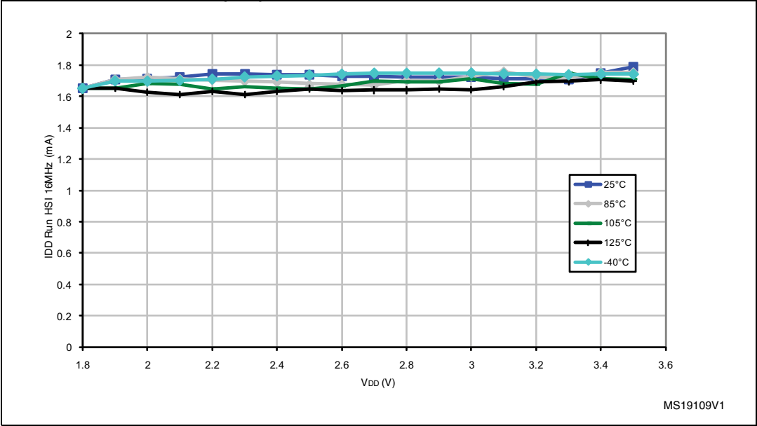
Figure 14. Typical I_{DD(RUN)} from RAM vs. V_{DD} (HSI clock source), f_{CPU} = 16\text{ MHz}
