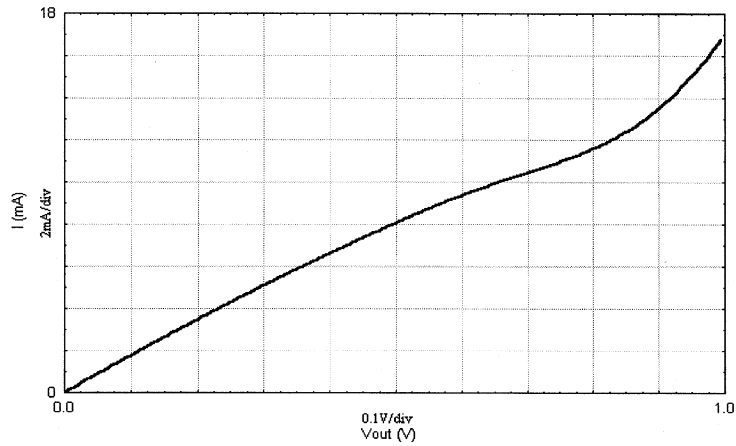
Figure 11. Output Sink Current vs. Output Voltage
