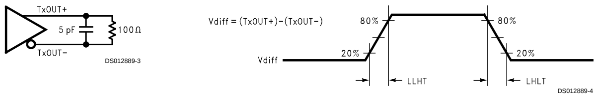
FIGURE 2. DS90CR283 (Transmitter) LVDS Output Load and Transition Timing
