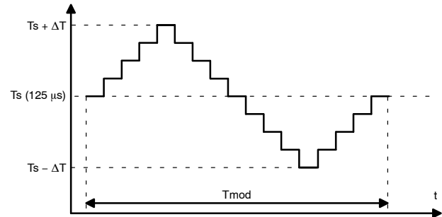
Figure 17. Spread Spectrum
