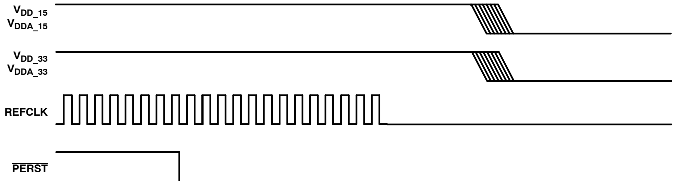
Figure 3–3. Power-Down Sequence
