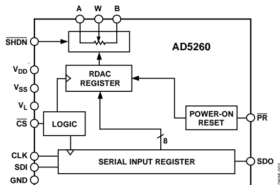
Figure 1. AD5260
