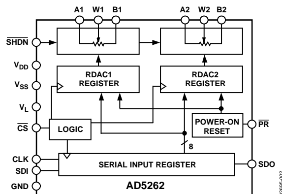
Figure 2. AD5262
