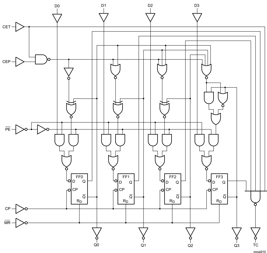
Fig 8. Logic diagram
