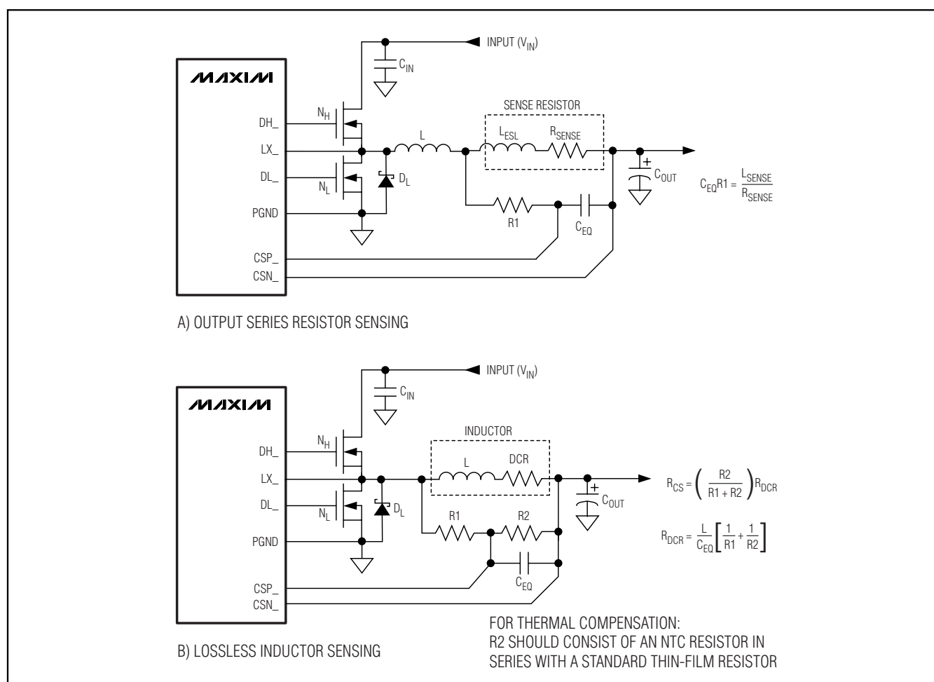
Figure 3. Current-Sense Methods
