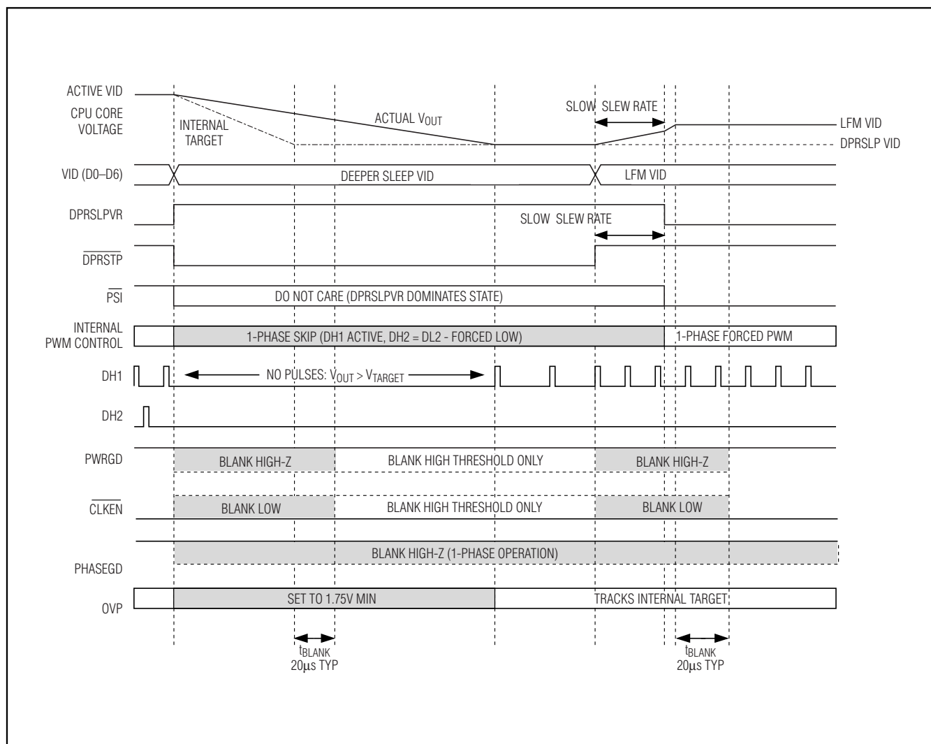
Figure 7. \overline{\text{PSI}} Transition
