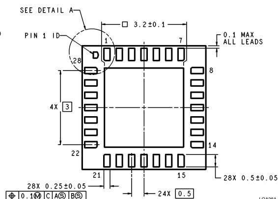
28-Pin Leadless Leadframe Package (LLP) NS Package Number LQA28A
