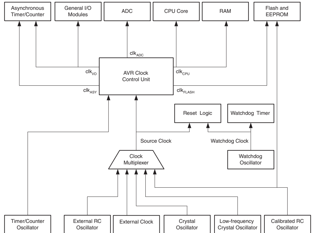
Figure 11. Clock Distribution
