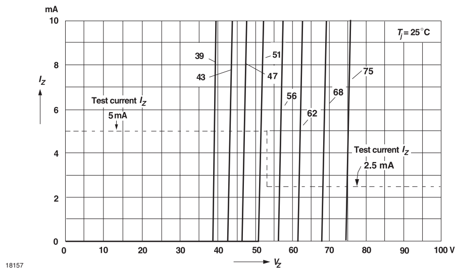
Fig. 16 - Breakdown Characteristics
