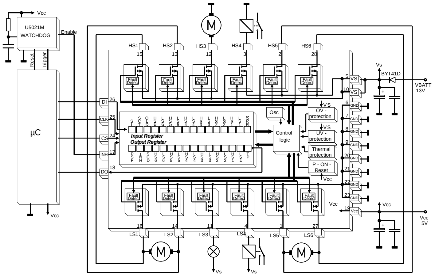
Figure 5. Application Circuit
