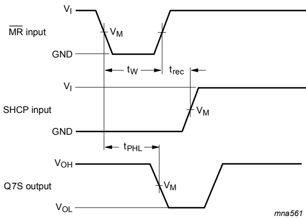
Measurement points are given in Table 16 . V_{OL} and V_{OH} are typical output voltage levels that occur with the output load. Figure 11. The master reset ( \overline{\text{MR}} ) pulse width, the master reset to serial data output (Q7S) propagation delays and the master reset to shift clock (SHCP) recovery time
