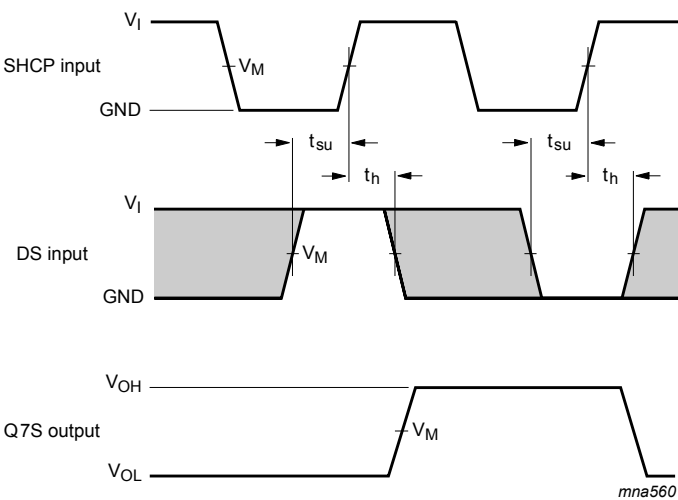
Measurement points are given in Table 16 . V_{OL} and V_{OH} are typical output voltage levels that occur with the output load. Figure 9. The data set-up and hold times for the serial data input (DS)
