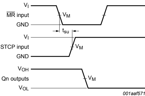
Measurement points are given in Table 16 . V_{OL} and V_{OH} are typical output voltage levels that occur with the output load. Figure 10. The master reset ( \overline{MR} ) to storage clock (STCP) set-up time
