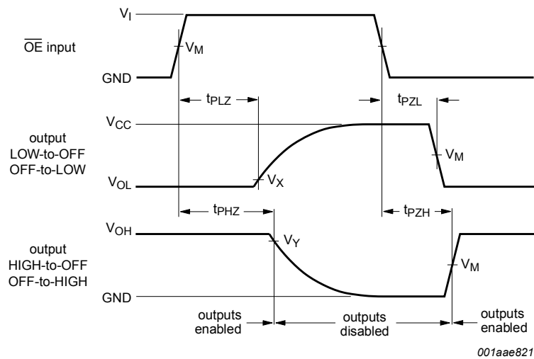
Measurement points are given in Table 16 . V_{OL} and V_{OH} are typical output voltage drops that occur with the output load. Figure 12. 3-state enable and disable times
