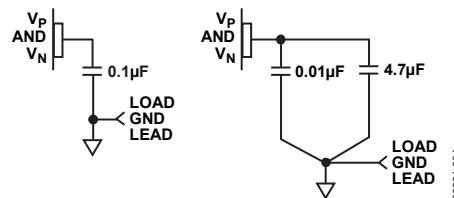
Figure 34. Supply Decoupling Options
