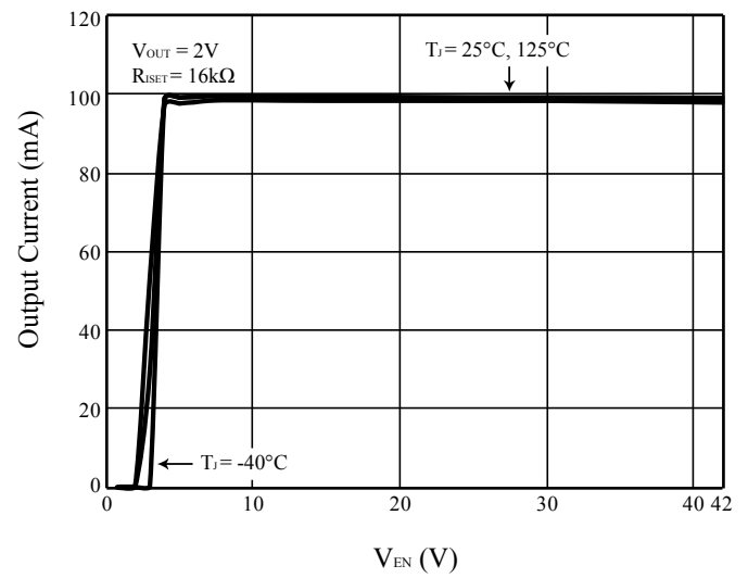
Figure 3 Output Current vs. V_{EN}
