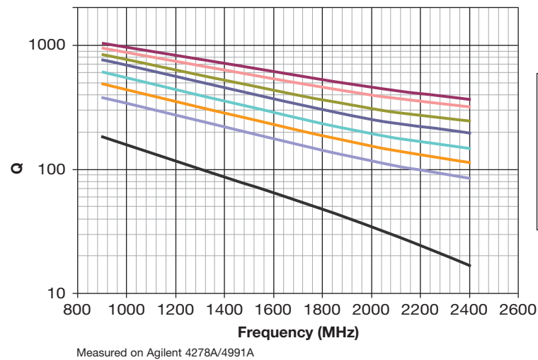
Accu-P® 1210 Typical Q vs Frequency
