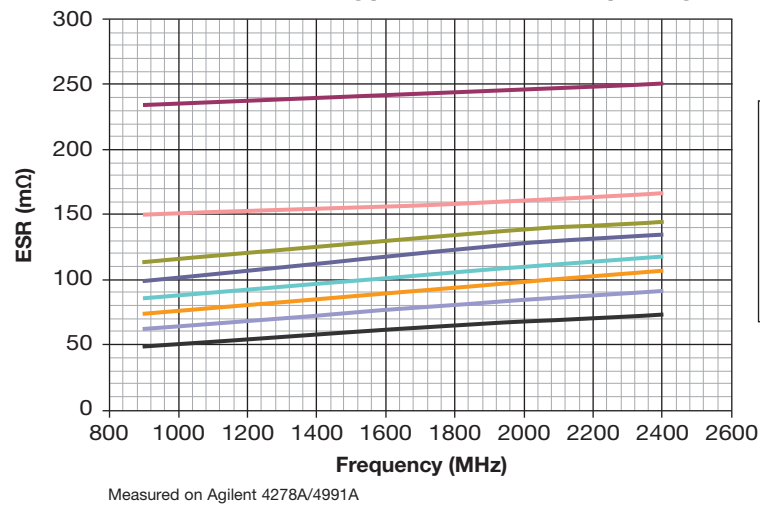
Accu-P® 1210 Typical ESR vs Frequency
