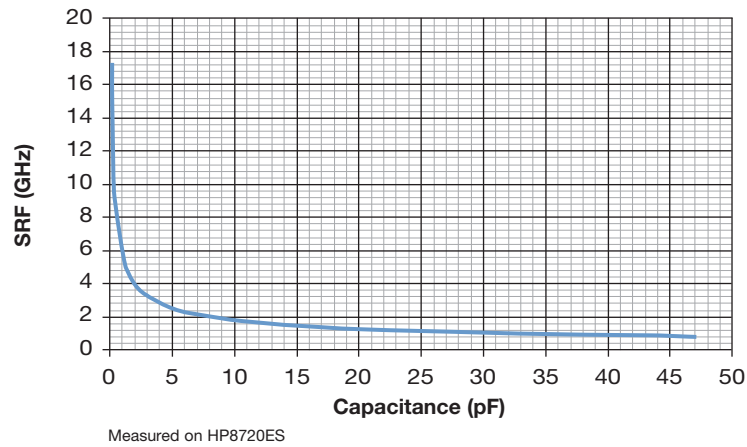
Accu-P® 1210 Typical SRF vs Capacitance
