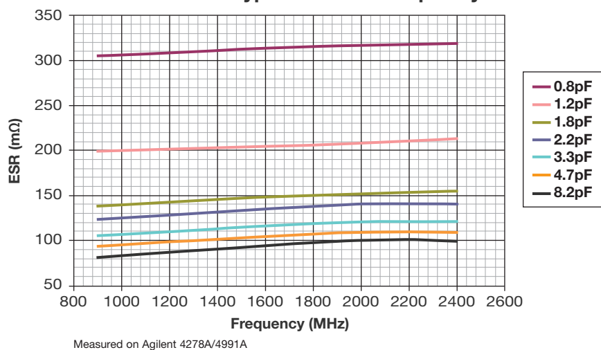
Accu-P® 0805 Typical ESR vs Frequency
