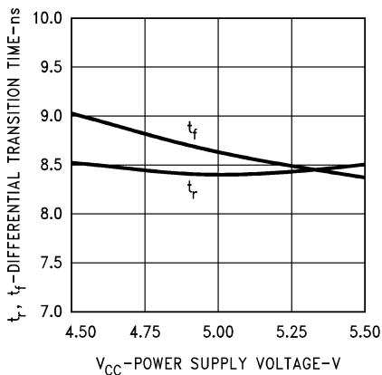
Driver Differential Transition Time vs V_{CC}
