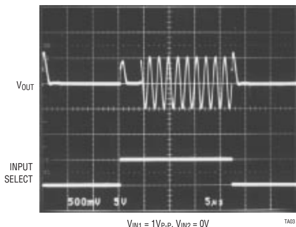
MUX Output
