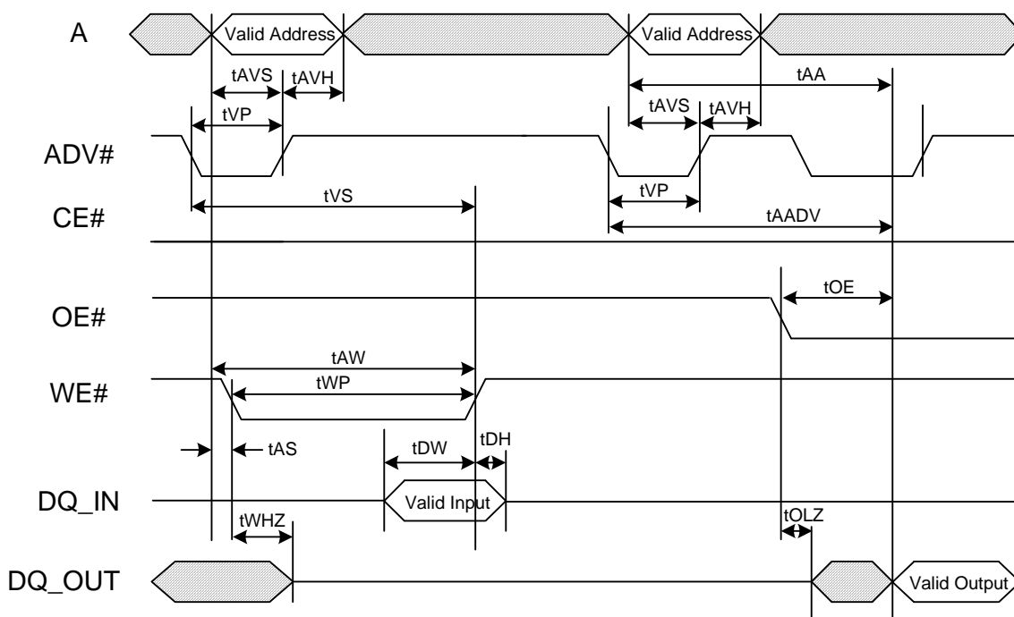
Figure 9. Asynchronous Write to Read Timing
