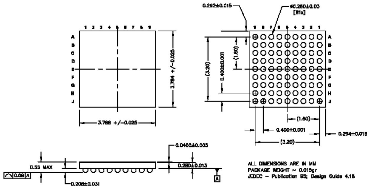
Figure 20. 81 WLCSP (3.784 × 3.788 × 0.55 mm)
