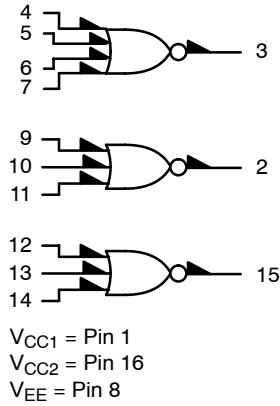
Figure 1. Logic Diagram
