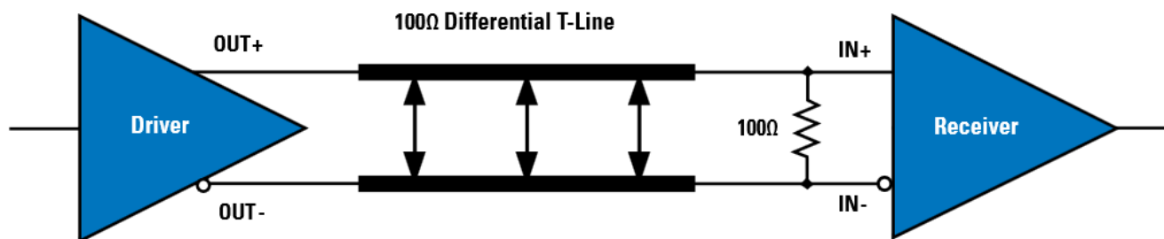
Figure 18. Point-to-Point Topology
