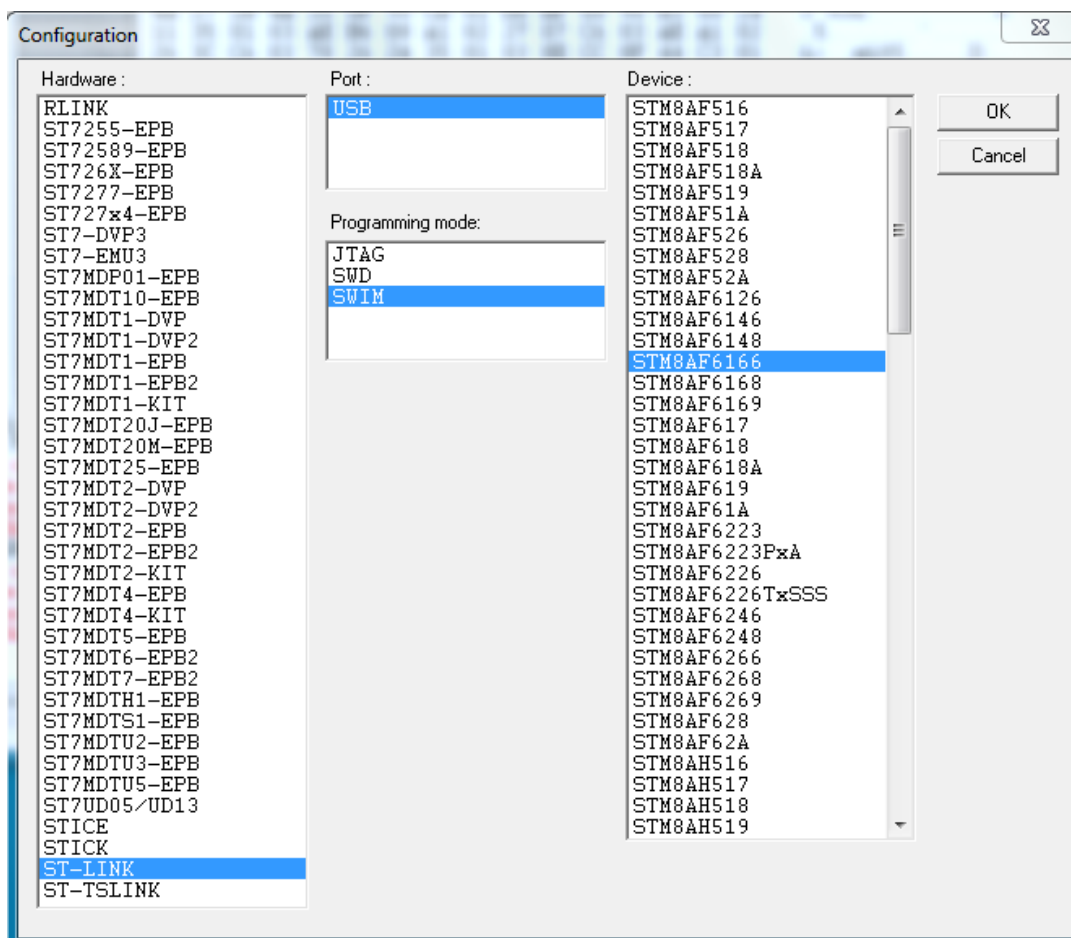
Figure 17. STVP configuration
