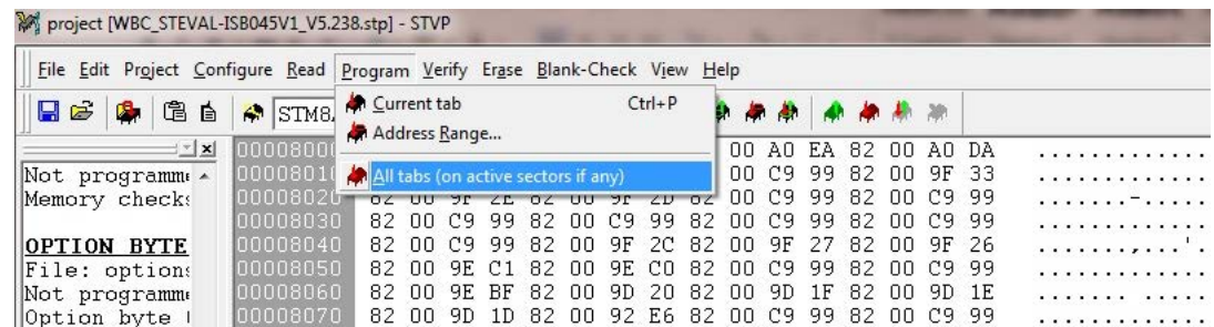
Figure 32. STVP download
