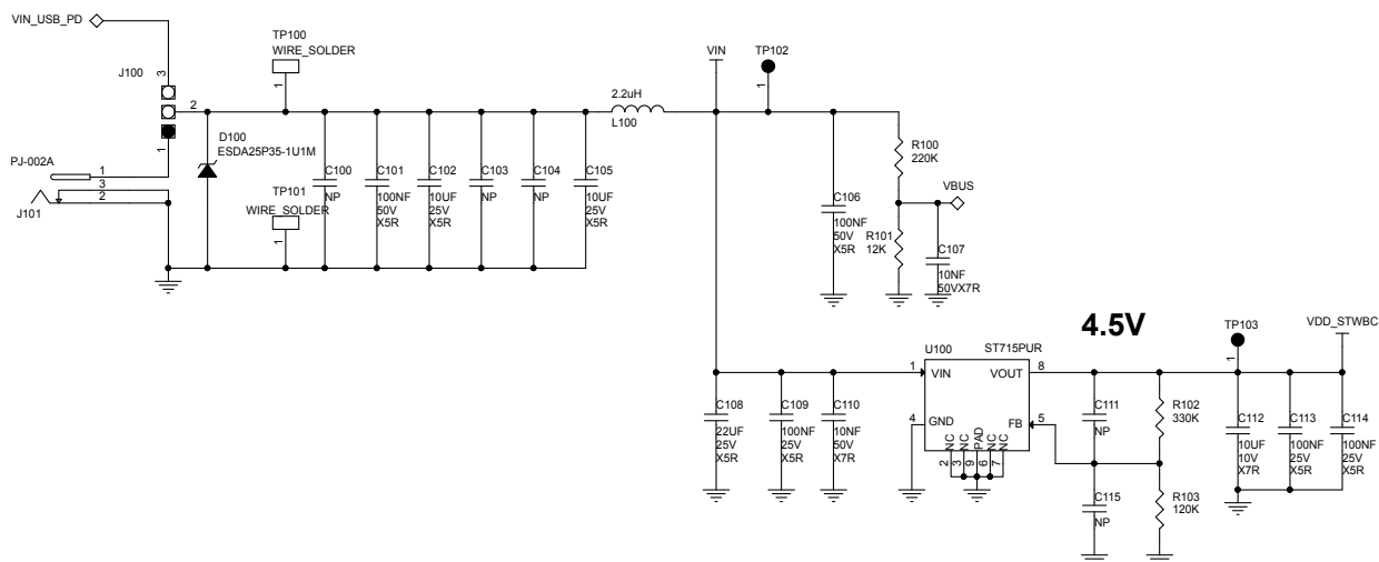
Figure 53. STEVAL-ISB047V1T - circuit schematic (supply)
