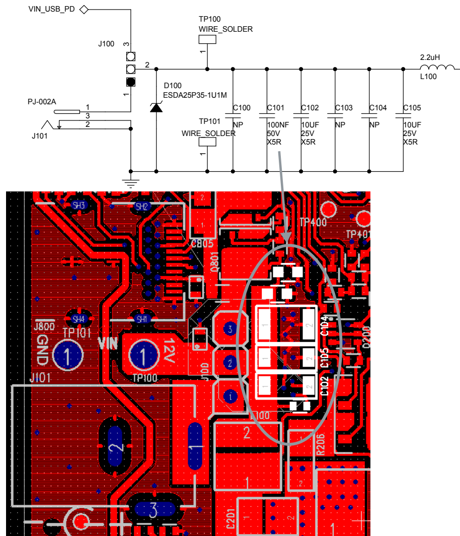
Figure 75. EMI components – 2
