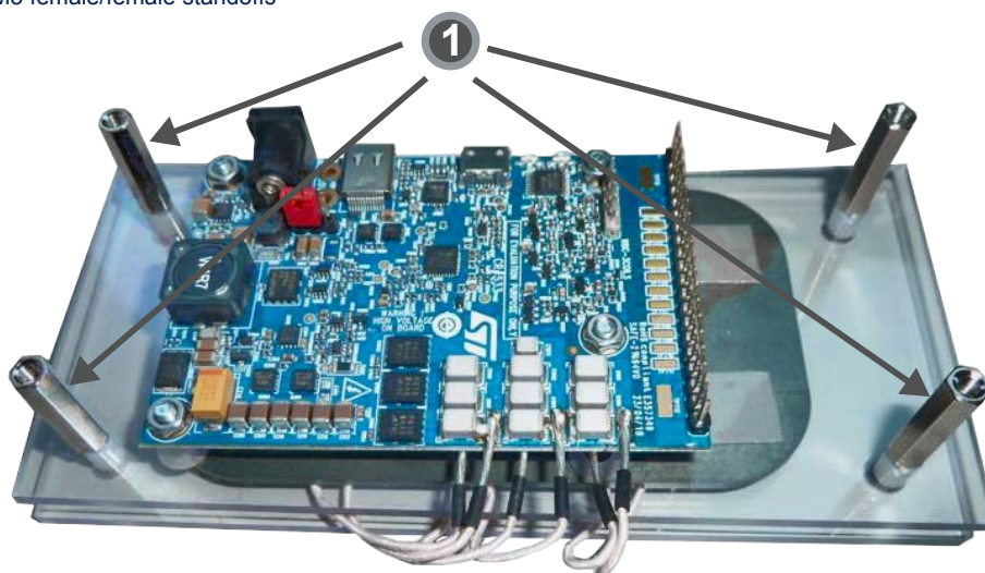
Figure 86. Final assembly
