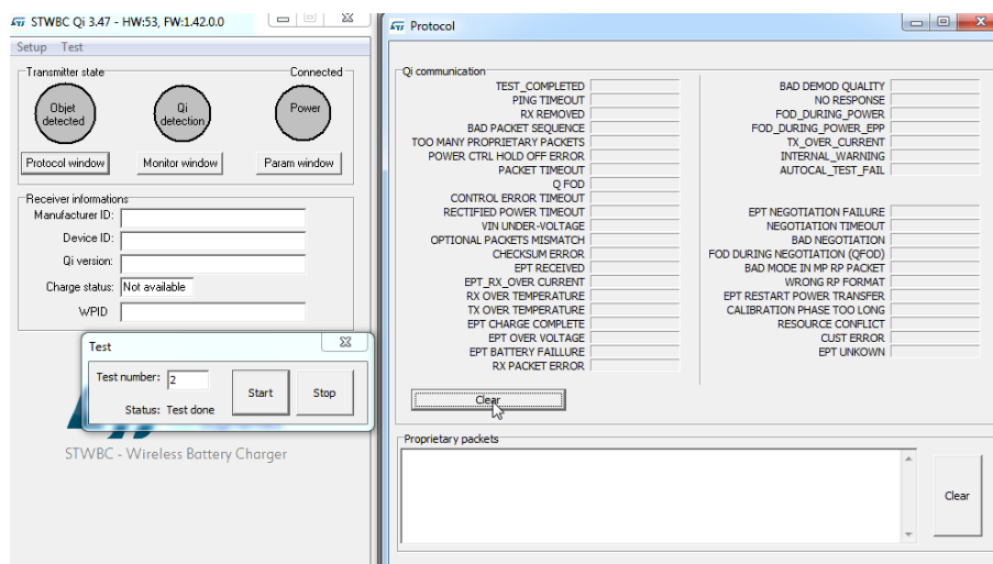
Figure 49. QFOD test
