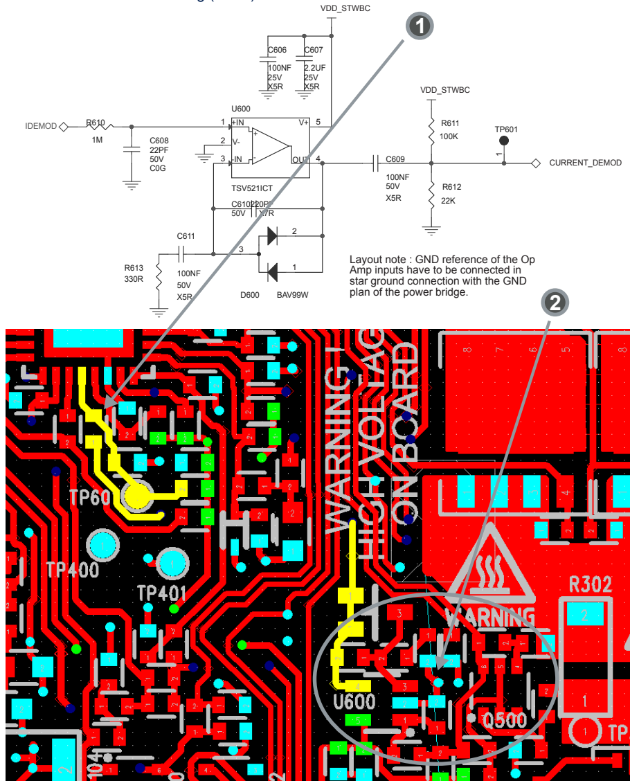
Figure 78. Current demodulation
