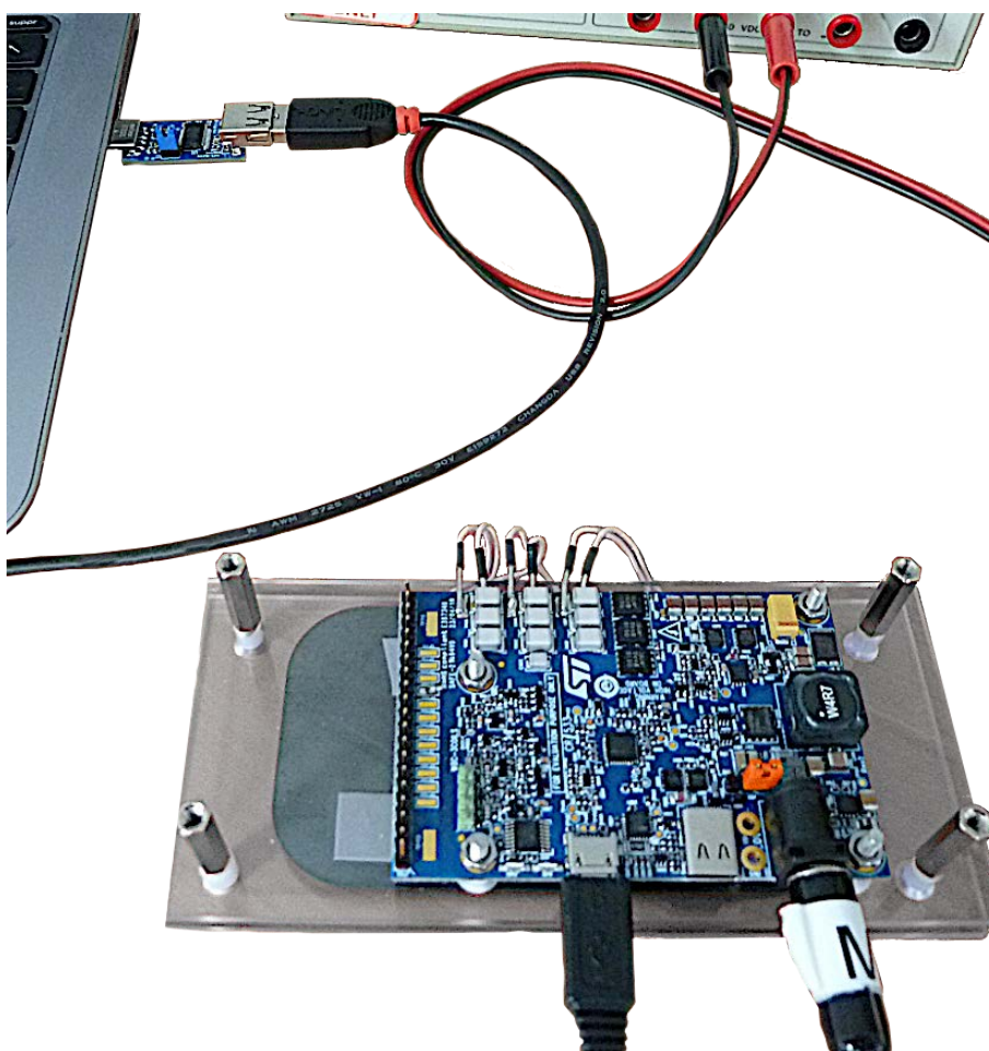
Figure 15. STEVAL-ISB047V1 evaluation kit connection
