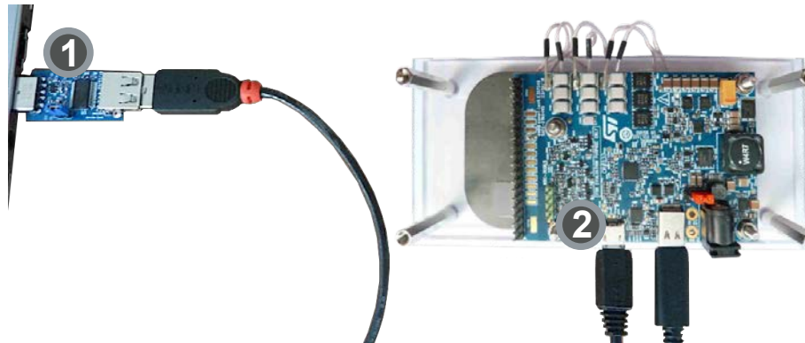
Figure 38. UART connection
