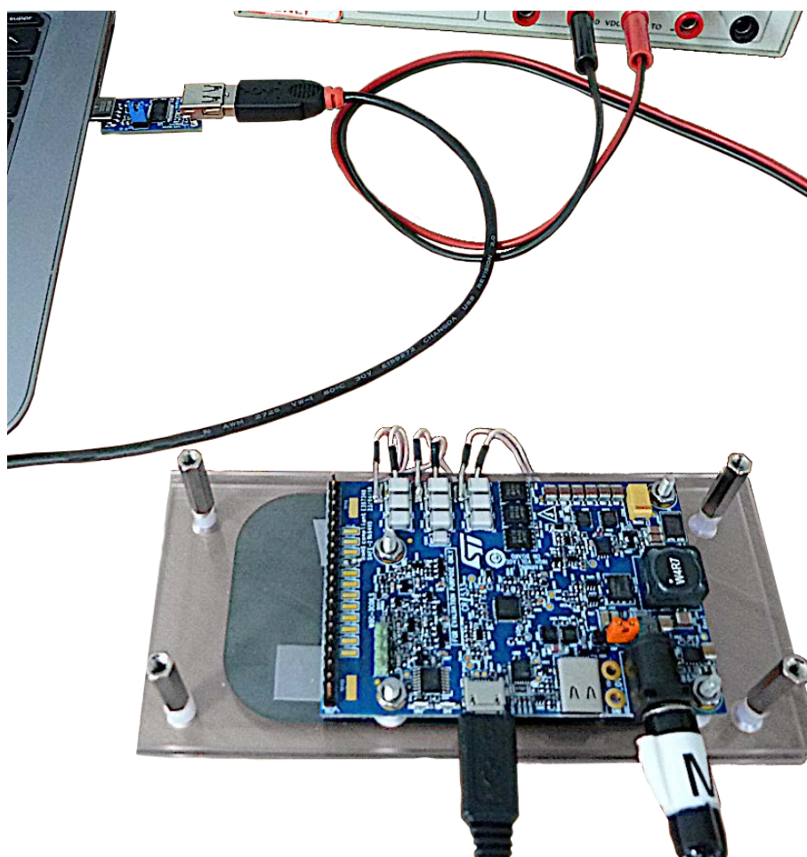
Figure 9. STEVAL-ISB047V1 evaluation kit connection
