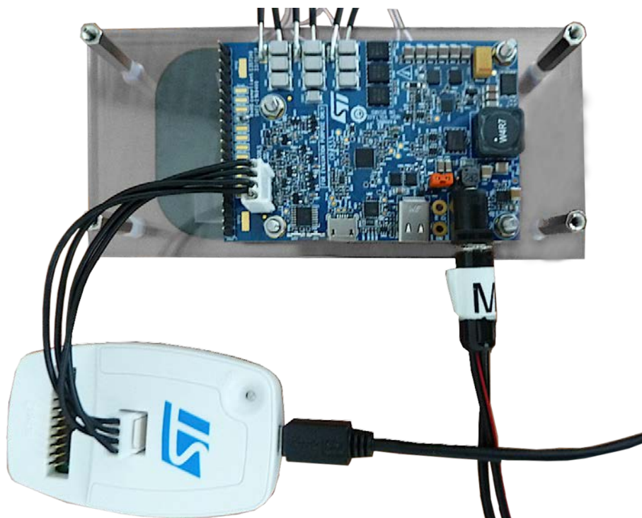
Figure 18. ST-LINK connection on the board
