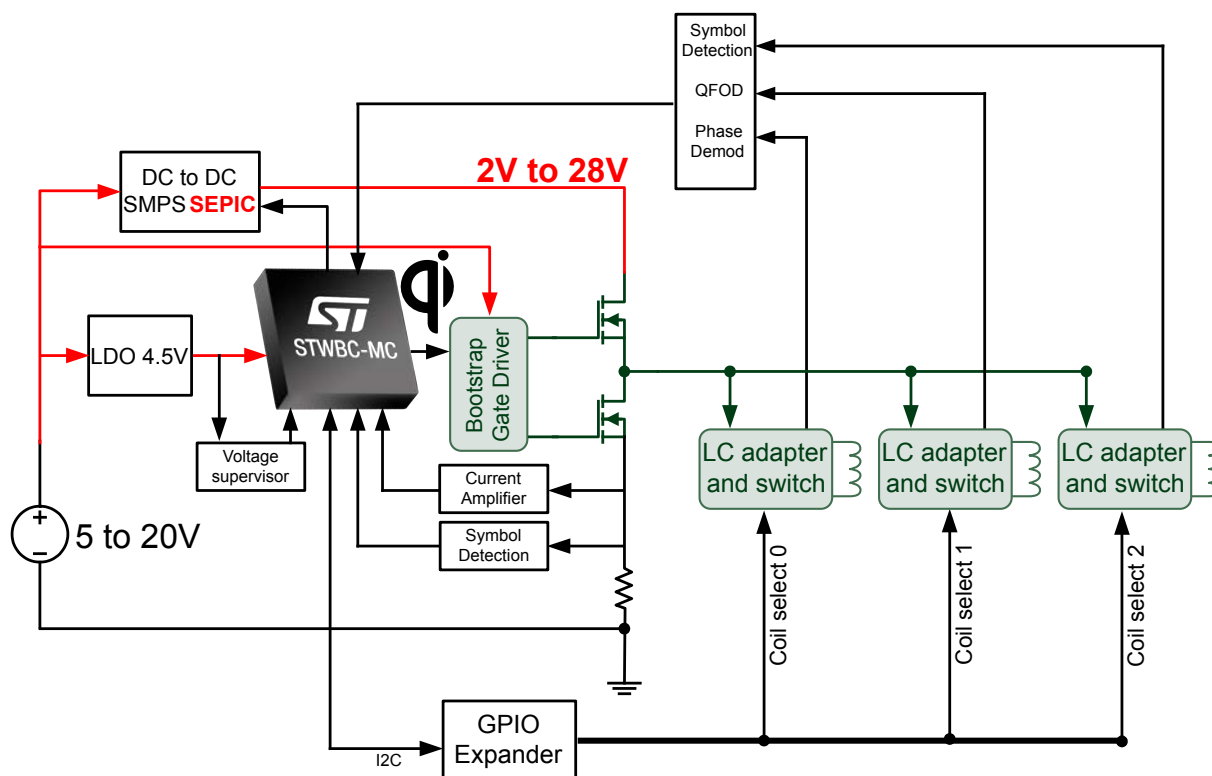
Figure 3. STEVAL-ISB047V1 block diagram
