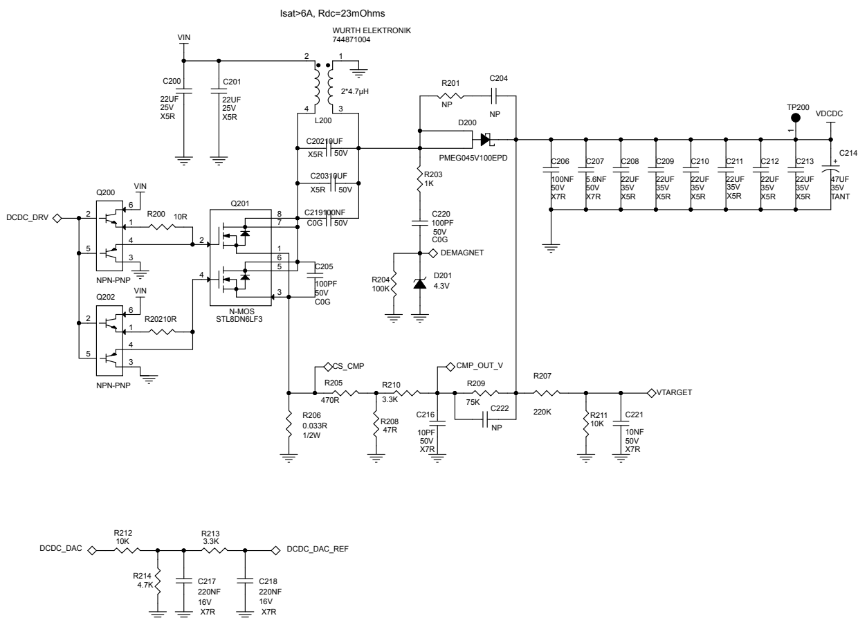
Figure 54. STEVAL-ISB047V1T - circuit schematic (sepic)
