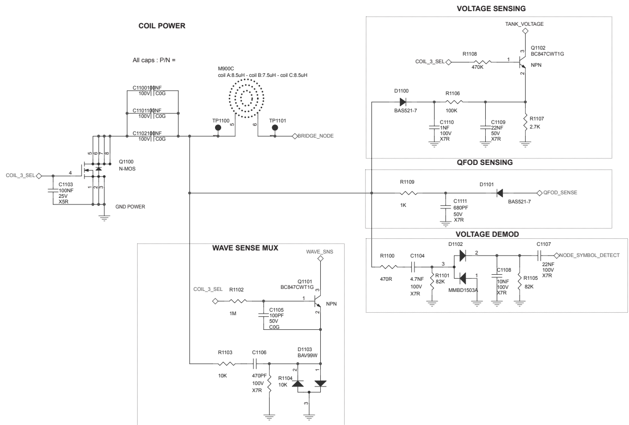
Figure 63. STEVAL-ISB047V1T - circuit schematic (coil3)
