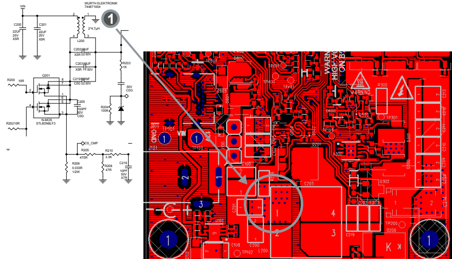
Figure 71. Details on SEPIC GND routing
