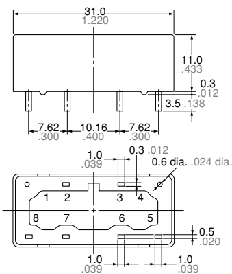
External dimensions
