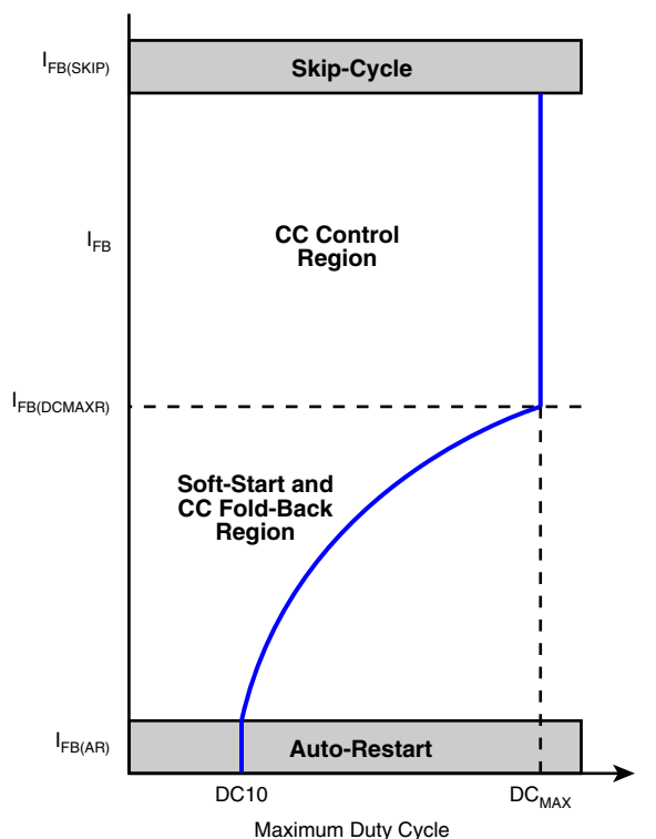
Figure 6. FEEDBACK Pin Current Characteristic.
