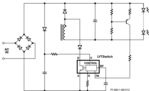
Figure 3b. Typical Buck Schematic.
