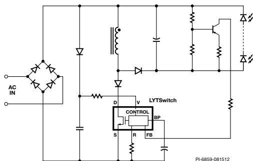
Figure 3d. Typical Buck-Boost Schematic.
