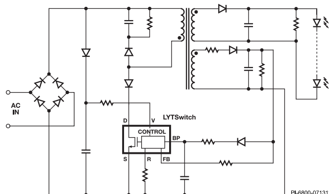
Figure 1. Typical Schematic.
