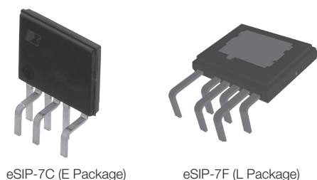
Figure 2. Package Options.
