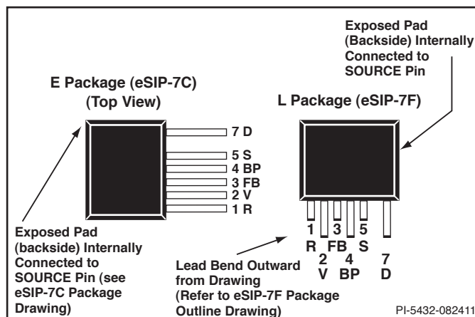
Figure 5. Pin Configuration.
