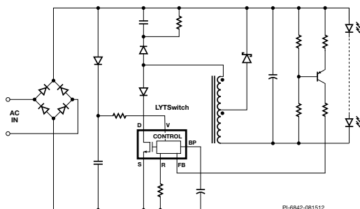
Figure 3c. Typical Tapped Buck Schematic.
