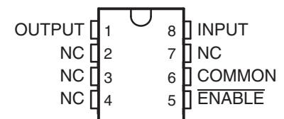
TL751L ... P PACKAGE (TOP VIEW)
