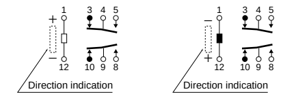
Schematic (Bottom view) Single side stable 1 coil latching
