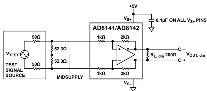
Figure 35. Basic Test Circuit
