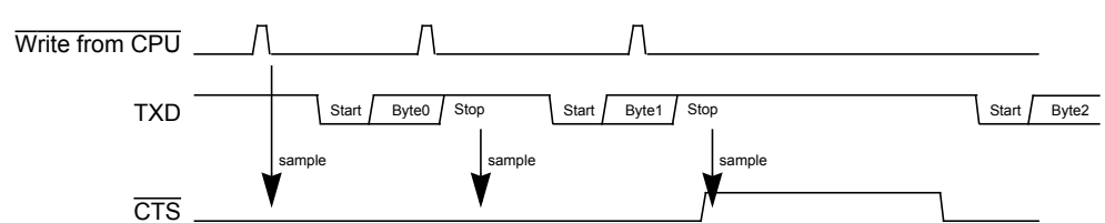
Figure 18-10. \overline{\text{CTS}} behavior
