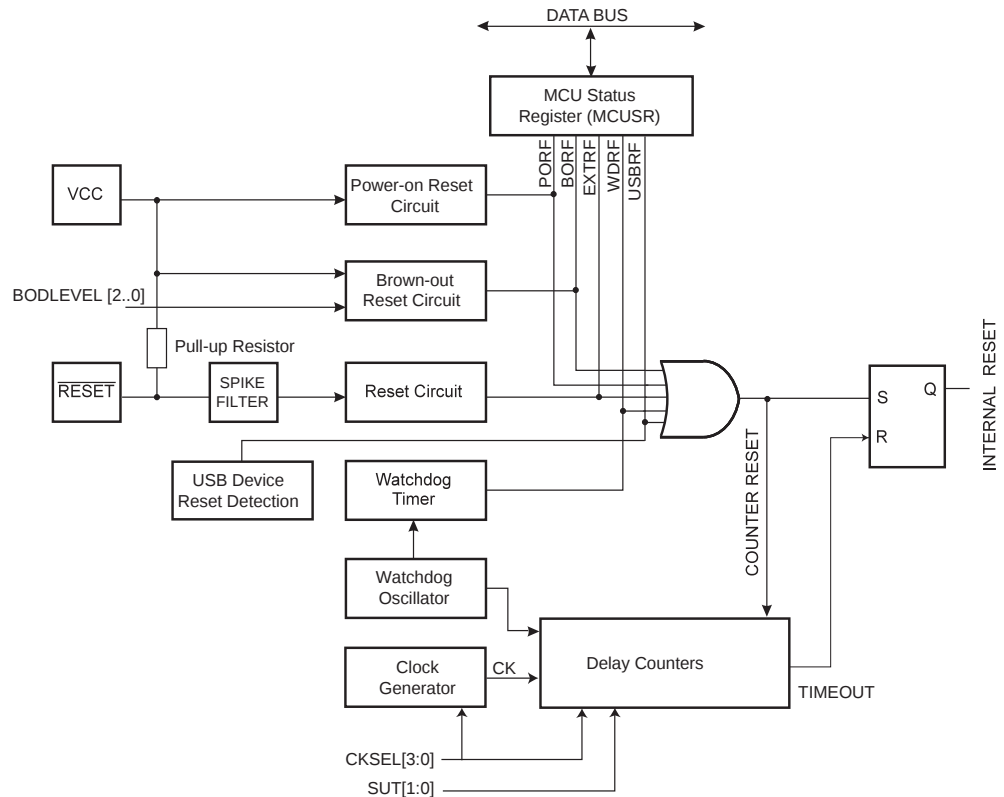
Figure 10-1. Reset Logic
