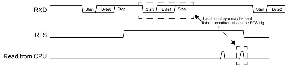
Figure 18-9. \overline{\text{RTS}} behavior
