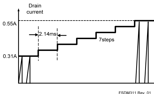
Figure 20. Internal Soft-Start
