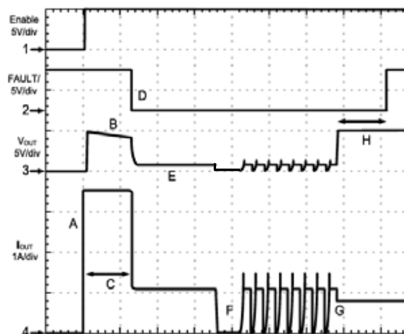
Figure 3. Kickstart Operation
