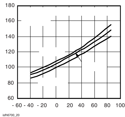
Fig. 20 - Typical Propagation Delays to Logic Low vs. Temperature (except SFH6705)
