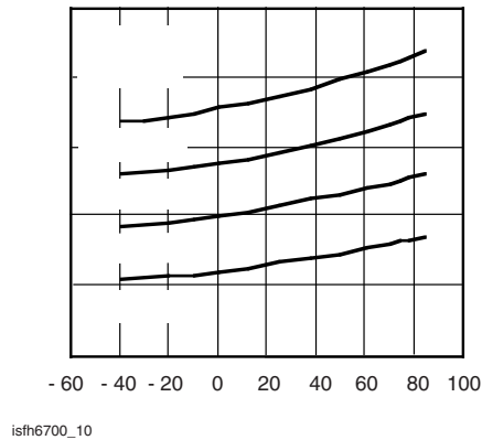
Fig. 10 - Typical Low Level Output Voltage vs. Temperature
