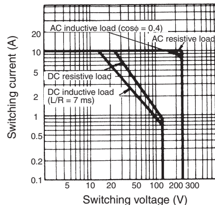
G4W-2212P-US-TV5
