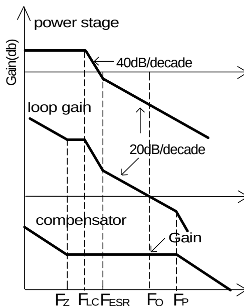
Figure 4 - Bode plot of Type II compensator
