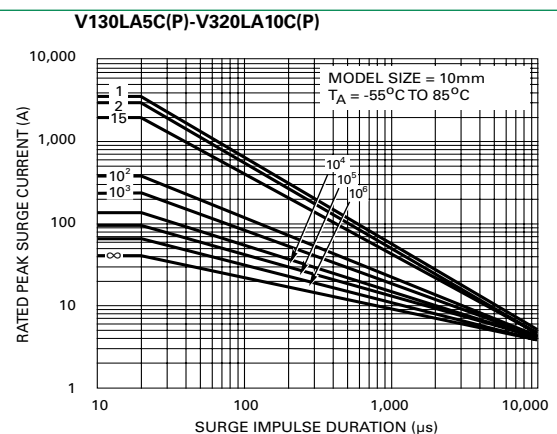
Figure 4. Repetitive Surge Capability for 10mm Parts
