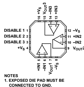
Figure 3. 16-Lead LFCSP_WQ
