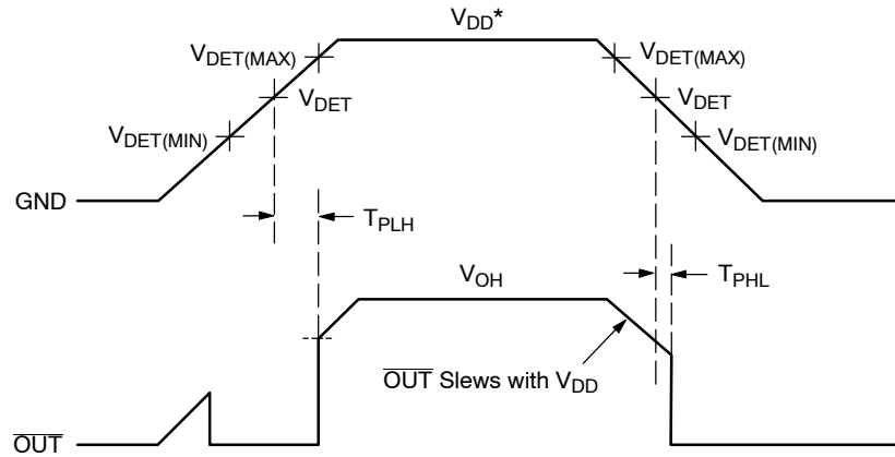
Figure 3. Timing Diagram
