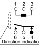
1-coil latching
