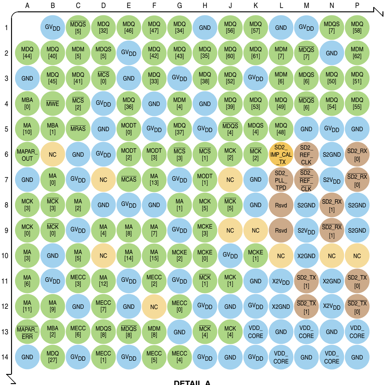
DETAIL A Figure 3. Chip Pin Map Detail A
