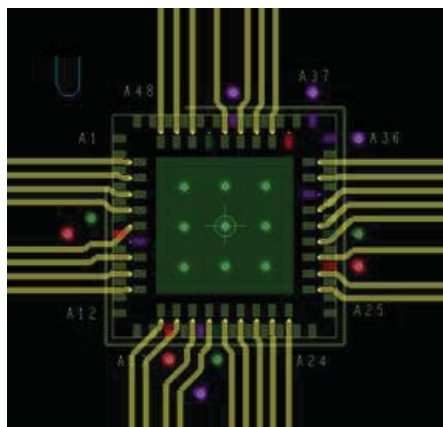
Figure 9. Bottom Layer
