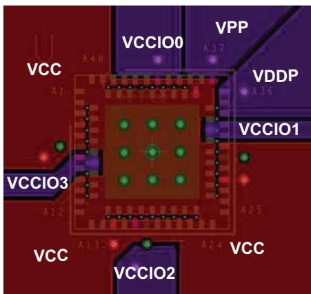
Figure 8. Power Layer
