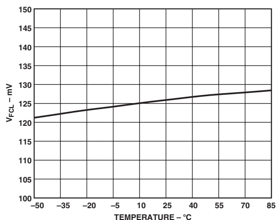
TPC 8. Fast Current Limit Voltage, V_{FCL} vs. Temperature
