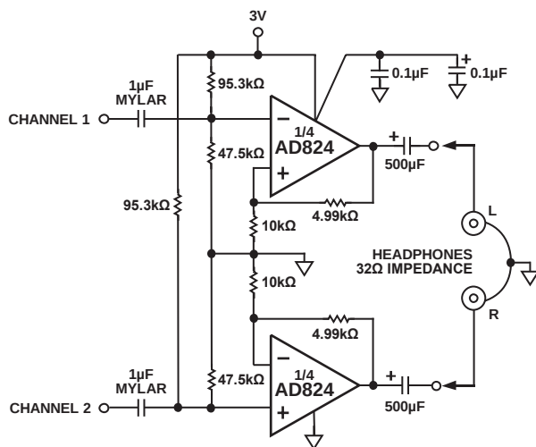
Figure 35. 3 Volt Single Supply Stereo Headphone Driver
